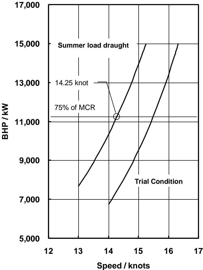
Figure 2.1: Power curves
